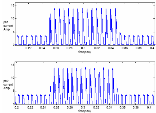
Fig. 8(b) Current profiles of phases 1 and 2 during load disturbance in sensorless mode
