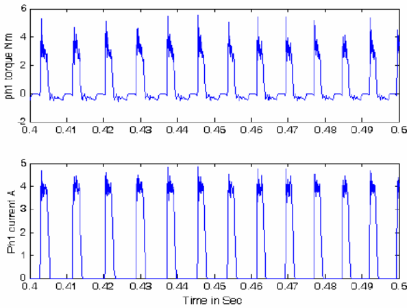
Fig. 6(b) Variation in phase current and torque during no load in sensorless mode
