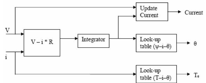
Fig. 4 Model for ‘Phase 1’ in sensor-less mode
